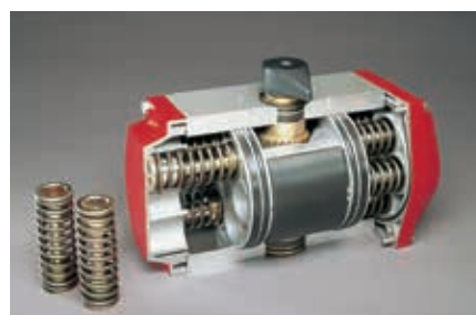
SPRING RETURN
