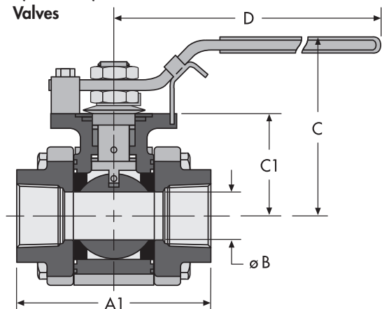
1/4" – 2 1/2" Valves
