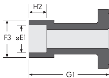
Flanged End Class 600 lb.
